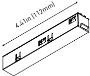
Live-End Connector 48V A338-00-01- | N | W |
